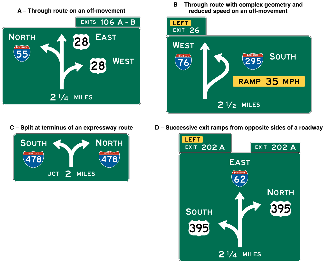
Figure 2E-41. Examples of Diagrammatic Advance Guide Signs
