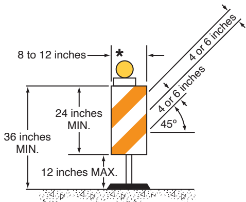
VERTICAL PANEL
