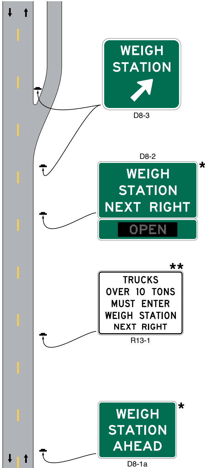
Figure 2D-23. Example of Weigh Station Signing – Conventional Road
